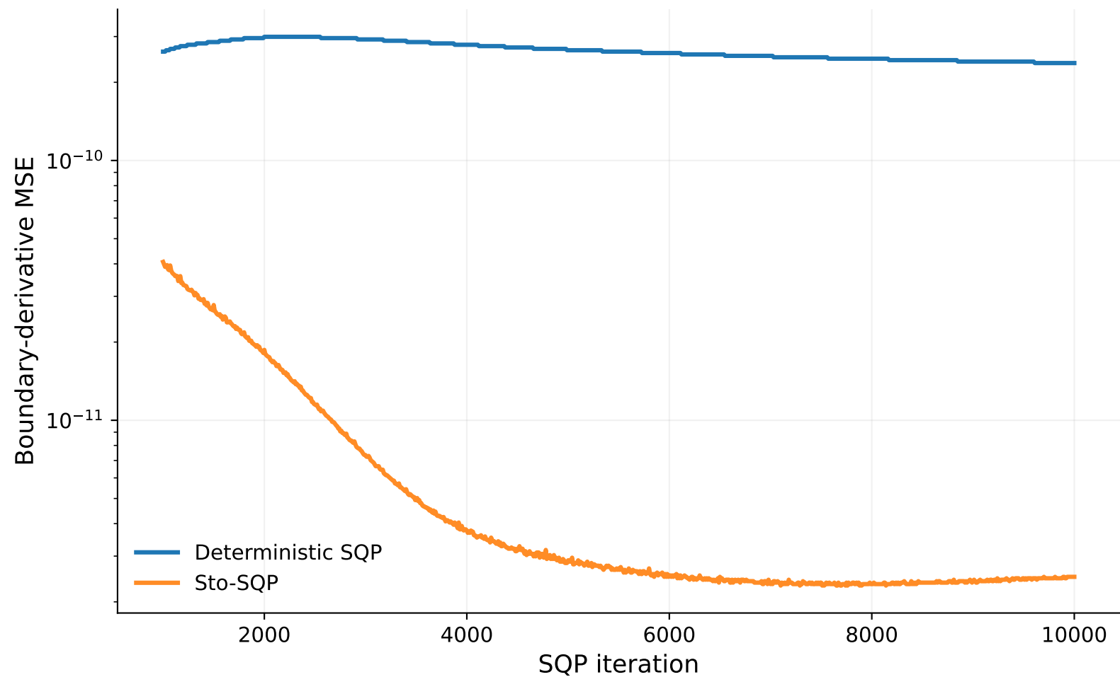
Burgers equation: boundary-derivative MSE — zoom: iter \geq 1000
