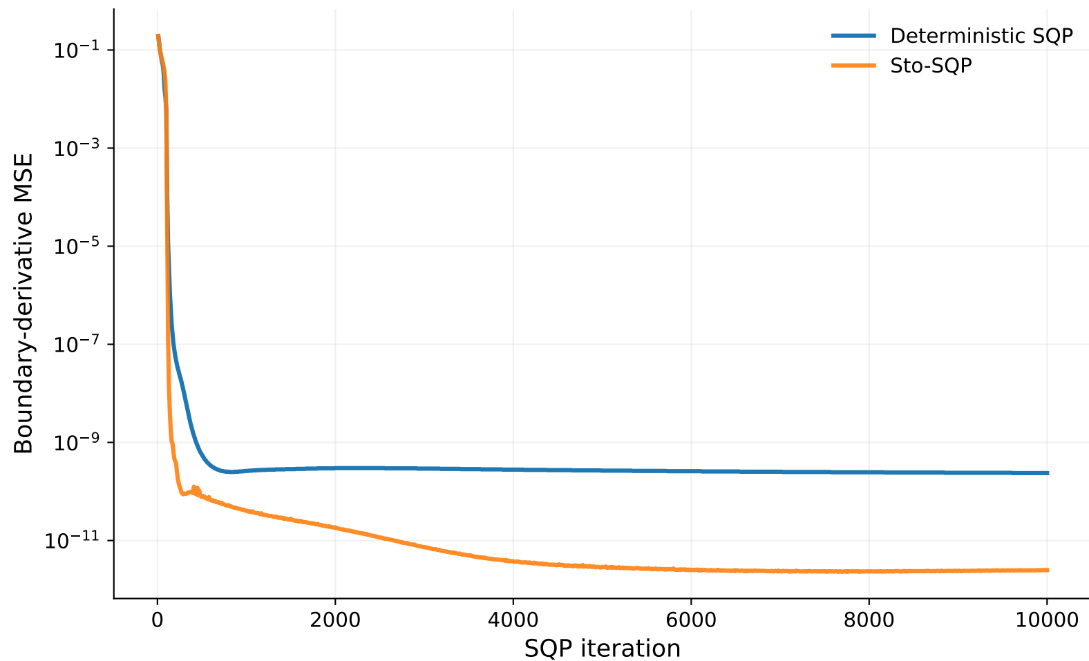
Burgers equation: boundary-derivative MSE — full trajectory
